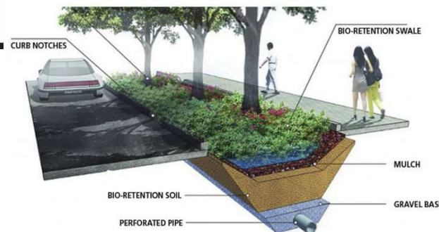
Section drawing of a rain garden
